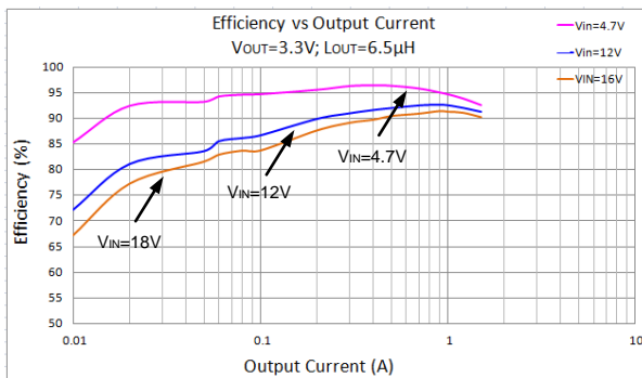
Figure 3. Efficiency (VOUT=3.3V)
