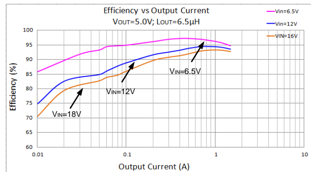
Figure 4. Efficiency (VOUT=5.0V)
