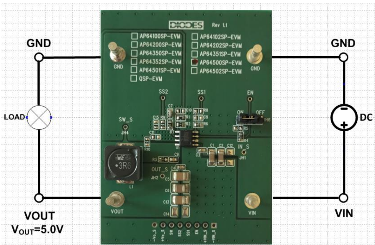
Figure 2. AP64500SP-EVM
