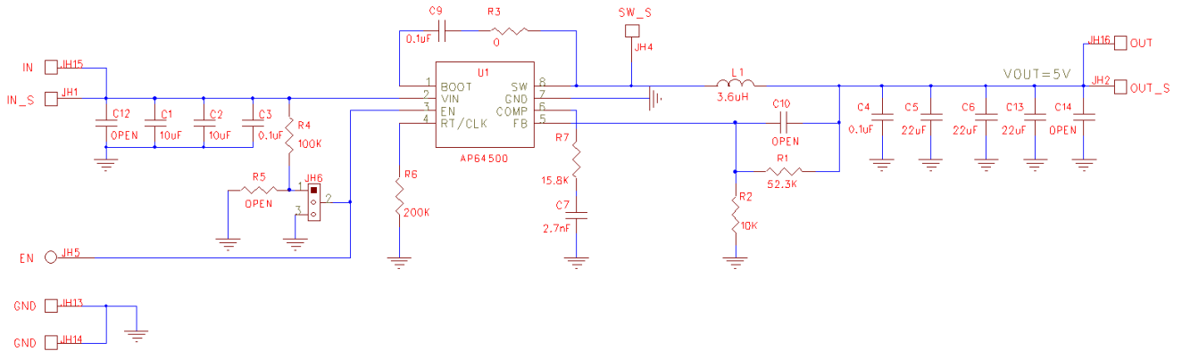
Figure 3. AP64500SP-EVM Schematic
