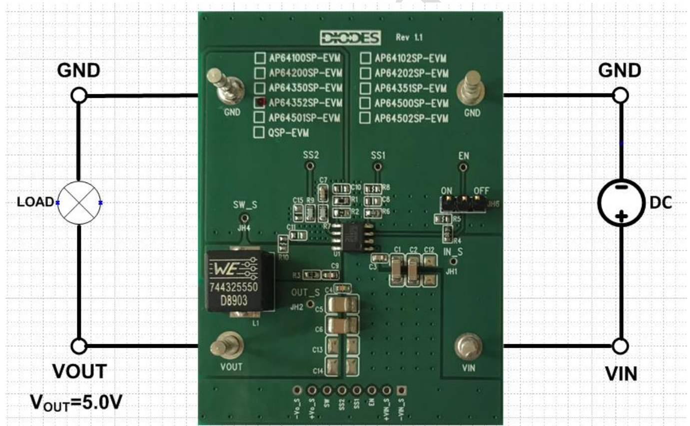
Figure 2. AP64352SP-EVM
