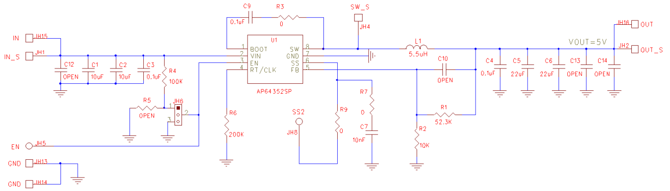
Figure 3. AP64352SP-EVM Schematic
