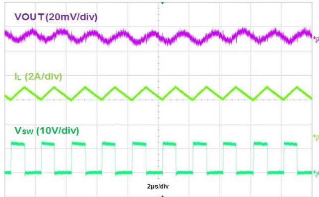
Figure 8. Output Voltage Ripple, IOU=3.5A
