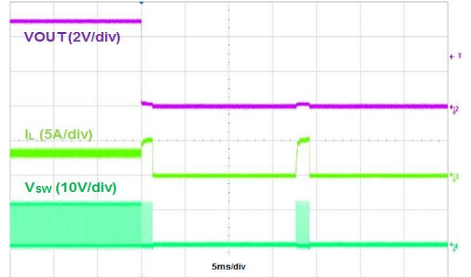
Figure 9. Output Short Protection, IOU=3.5A
