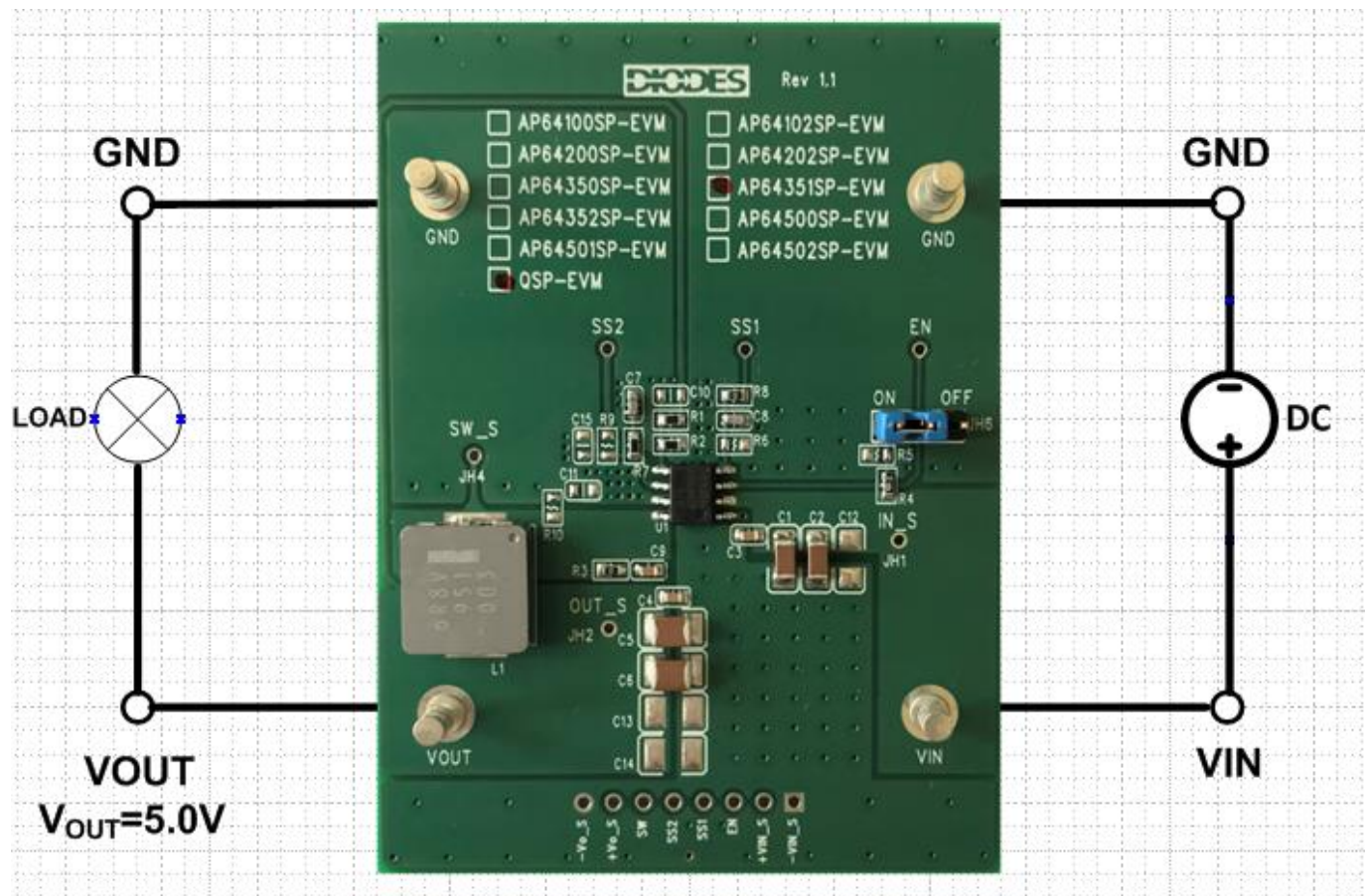
Figure 2. AP64351QSP-EVM
