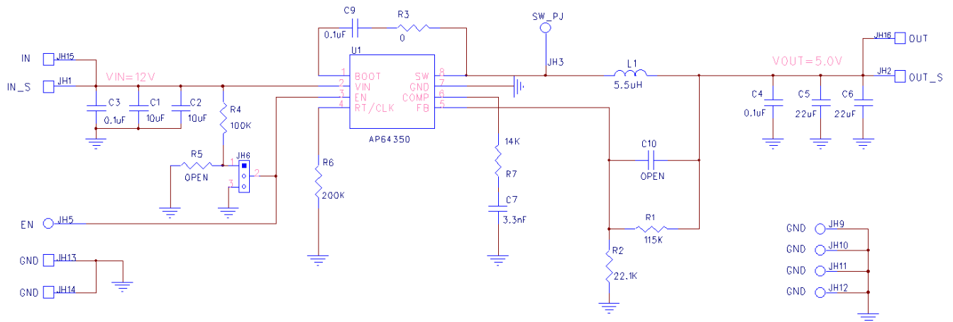
Figure 2. AP64350SP-EVM Schematic
