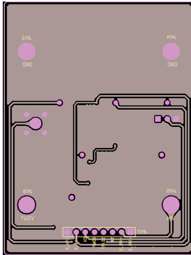
Figure 4. AP64350SP-EVM – Bottom Layer
