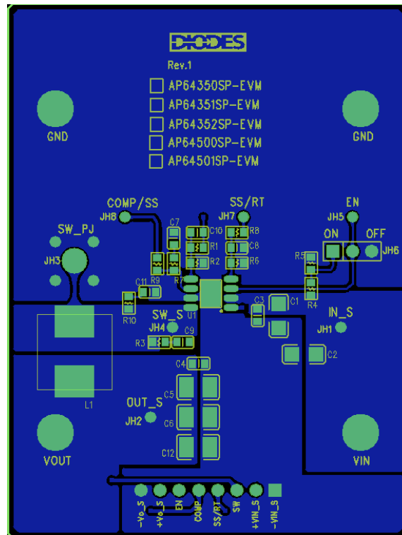
Figure 3. AP64350SP-EVM – Top Layer
