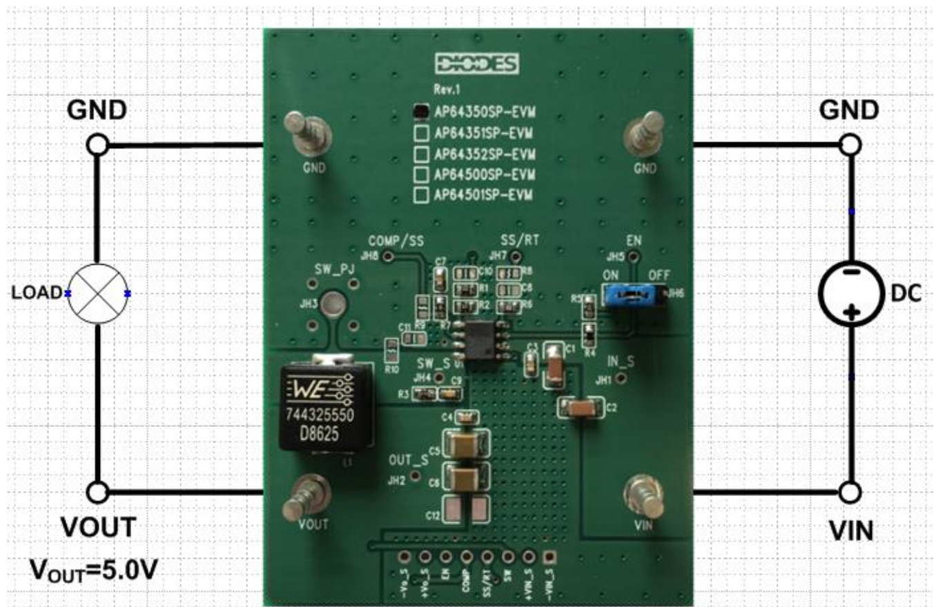
Figure 1. AP64350SP-EVM
