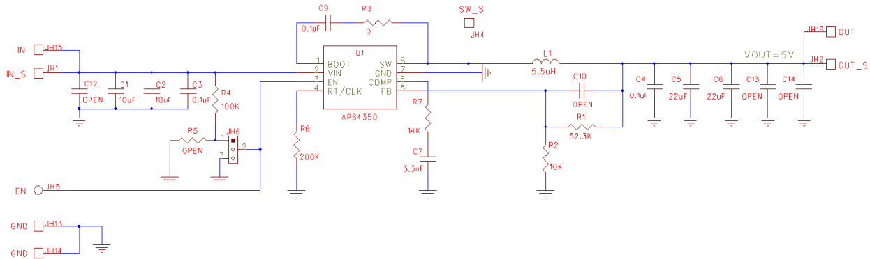
Figure 3. AP64350SP-EVM Schematic
