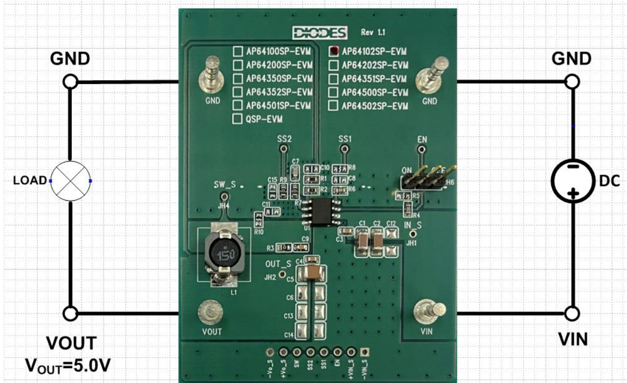
Figure 1. AP64102SP-EVM
