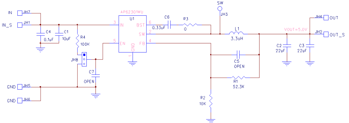
Figure 2. AP62301WU-EVM Schematic
