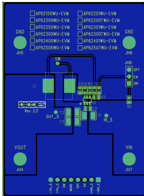
Figure 3. AP62301WU-EVM – Top Layer
