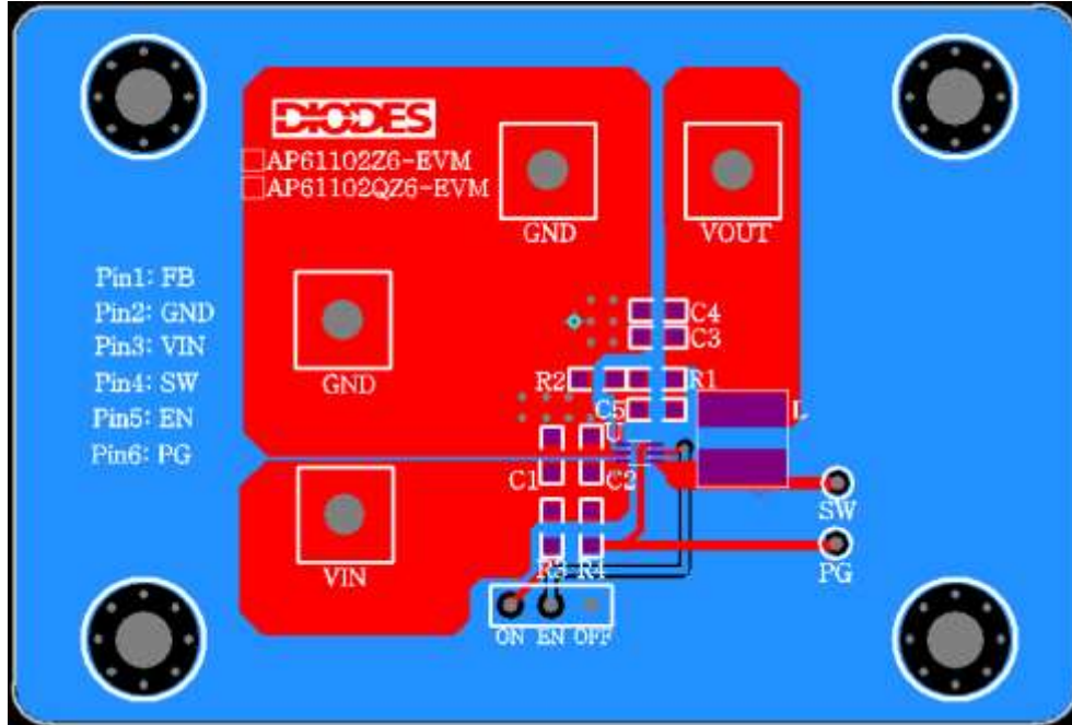
Figure 3. AP61102QZ6 - EVM - Top Layer
