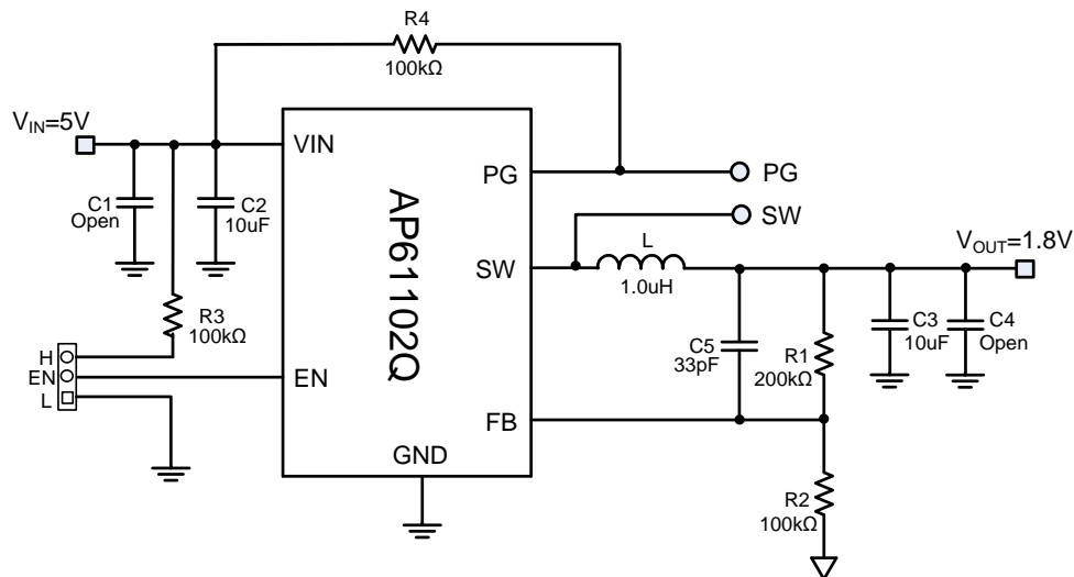
Figure 2. Typical Application Circuit (Vo=1.8V)
