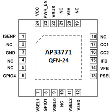
Figure 2 – Package Outline
