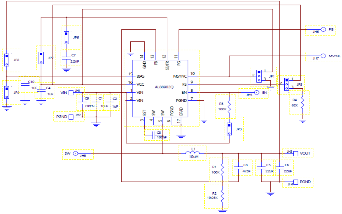
Figure 6: Schematic Circuit
