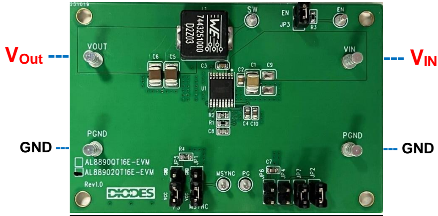
Figure 1: AL88902QT16E EVM Top View
