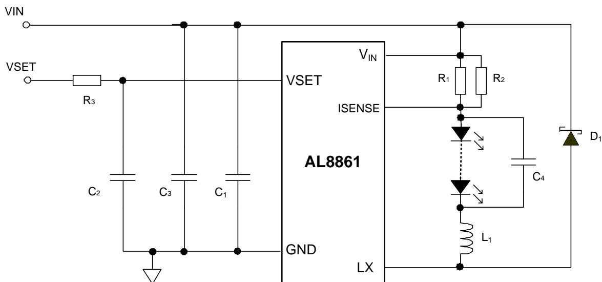
Figure 2: Schematic diagram
