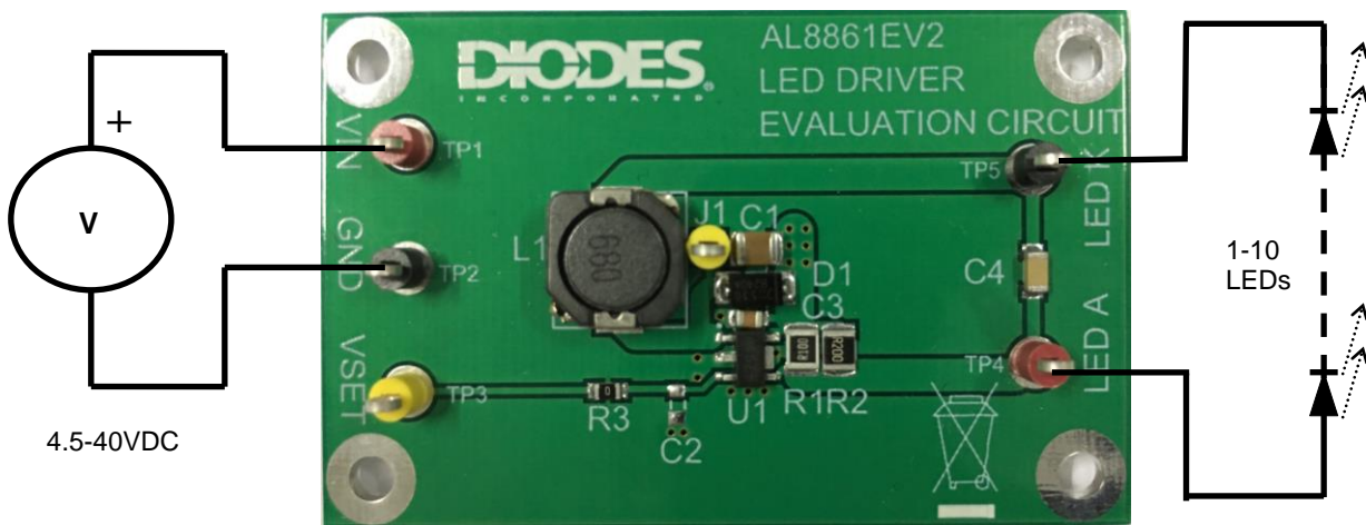
Figure 1: AL8861EV2 evaluation board and connection diagram
