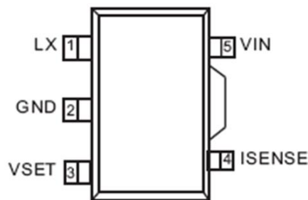
SOT89-5 package
