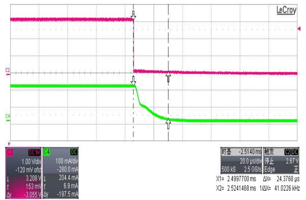
Figure 13. PWM Turn Off Delay
