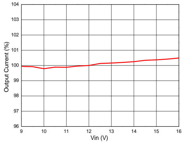
Relative Output Current vs. Vin
