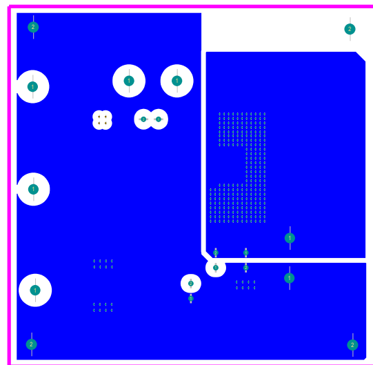
Figure 5. PCB Bottom Layer View
