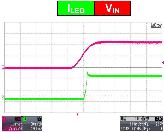
Figure 7. Low Side Startup
