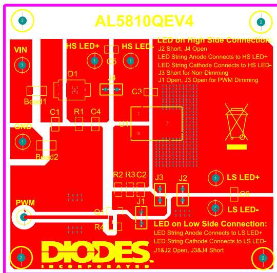
Figure 4. PCB Top Layer View
