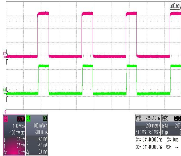
Figure 10. PWM Duty=25%
