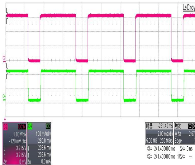
Figure 11. PWM Duty=75%
