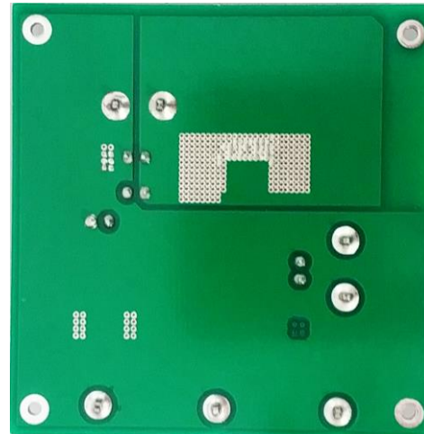
Figure 2. Bottom View
