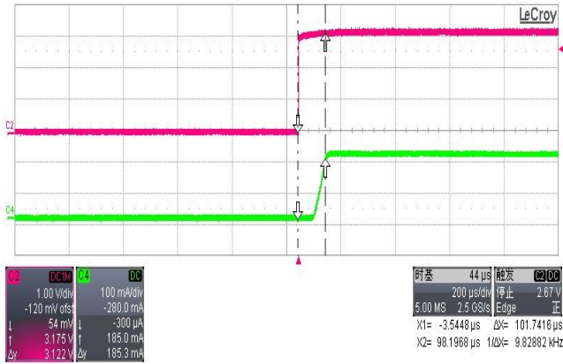
Figure 12. PWM Turn On Delay
