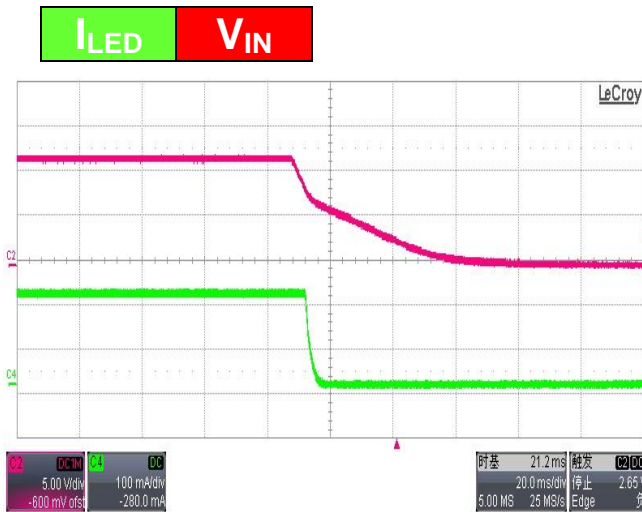
Figure 8. High Side Turn OFF
