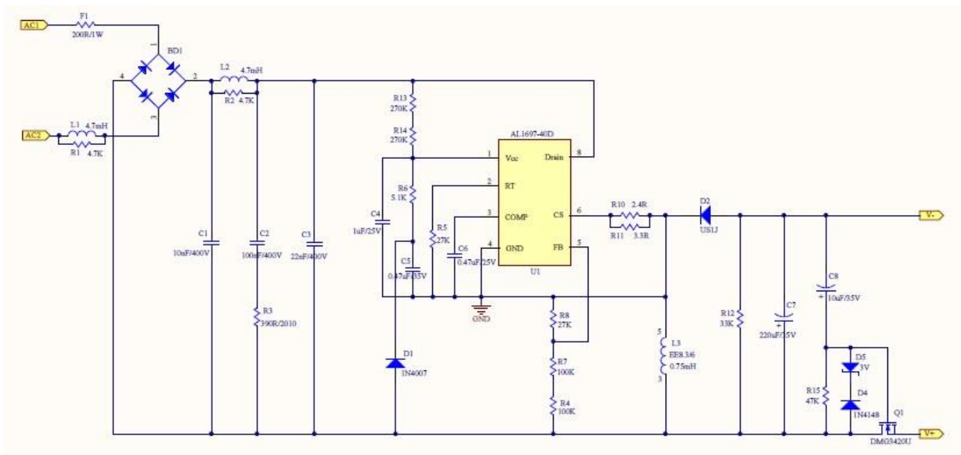
Figure 5: Schematic Circuit
