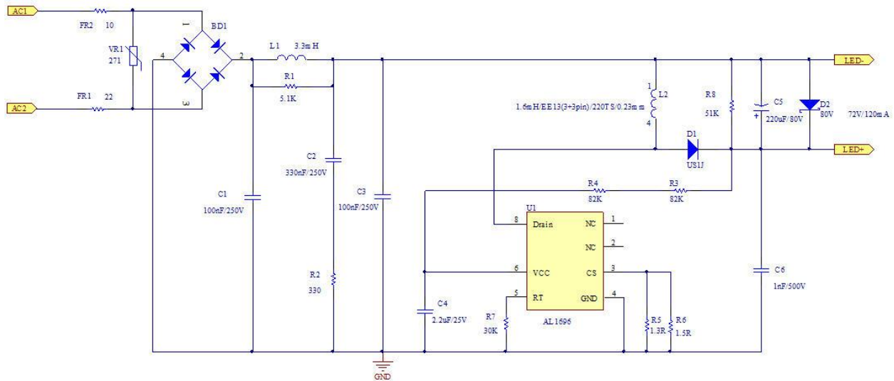
Figure 5: Schematic Circuit
