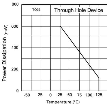
Power Derating
