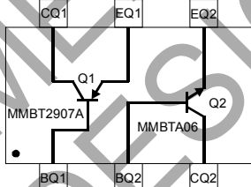
Device Schematic
