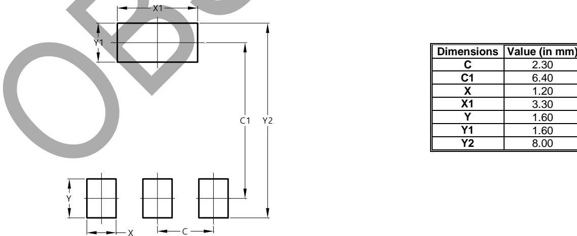
SOT223 (Type DN)
