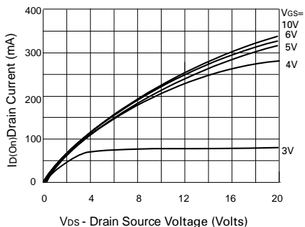
Saturation Characteristics
