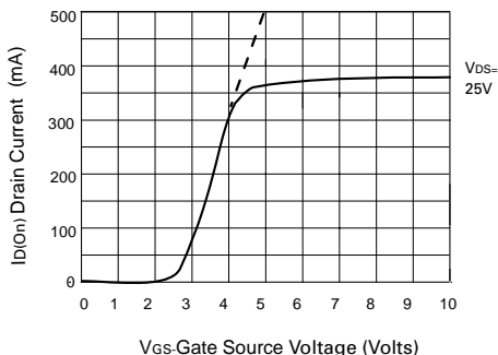
Transfer Characteristics
