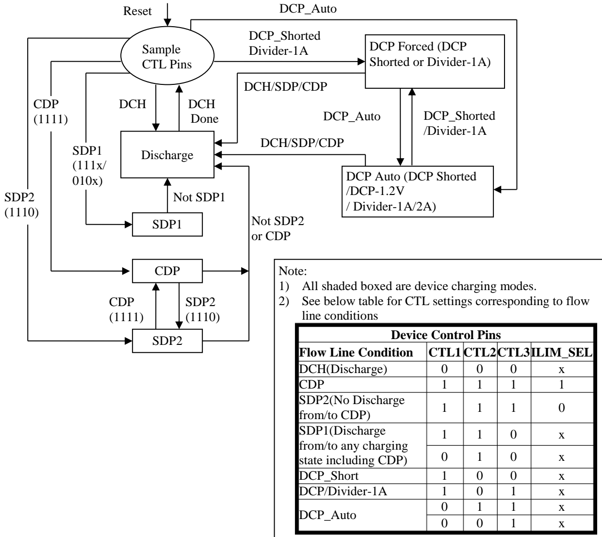
Figure 5, PI5USB2544Q Charging States
