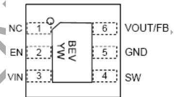
Top View DFN 2x2 6L
