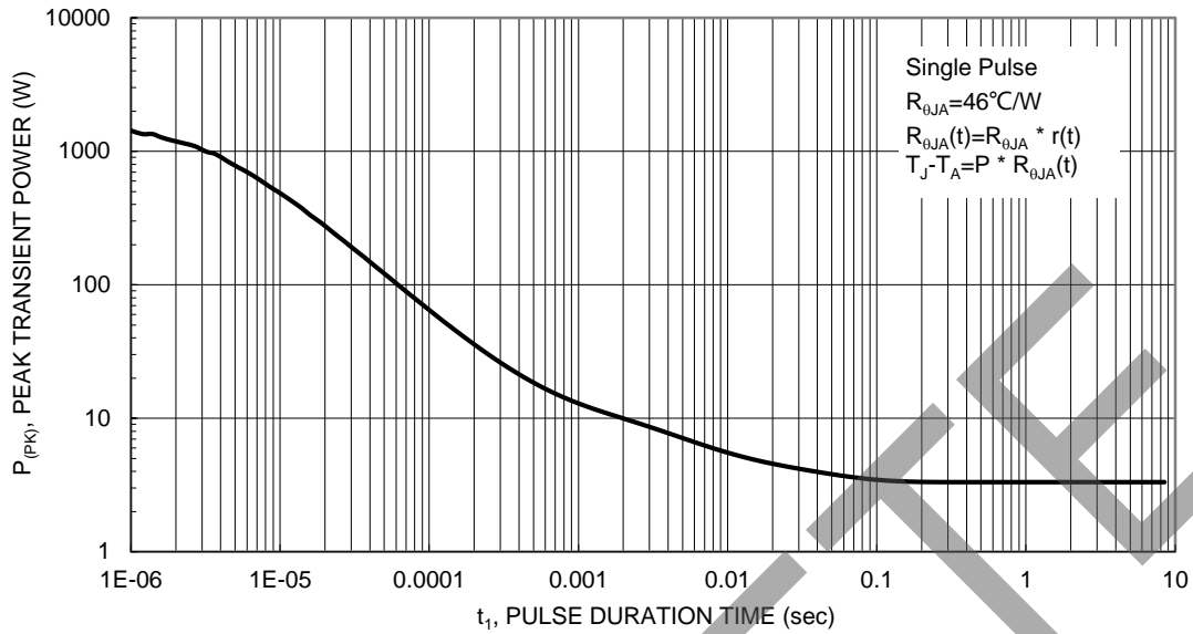
Figure 7. Single Pulse Maximum Power Dissipation
