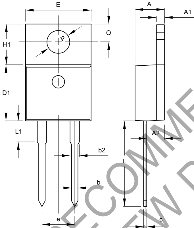
TO220AC (Type HE) (Future Release)
