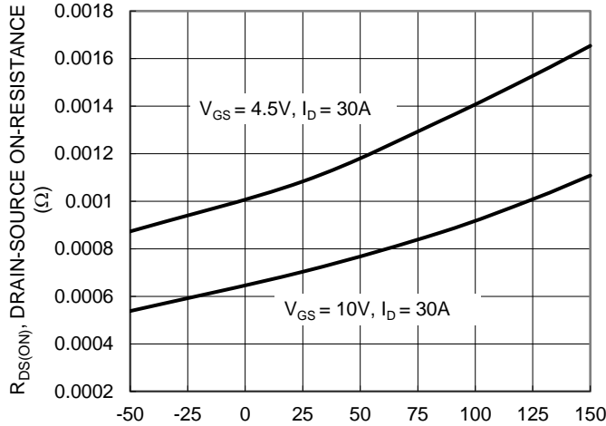
T J , JUNCTION TEMPERATURE (°C) Figure 7. On-Resistance Variation with Junction Temperature
