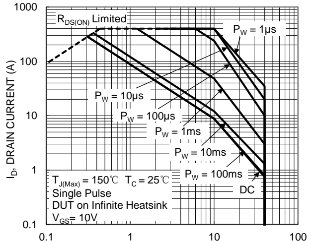
V DS , DRAIN-SOURCE VOLTAGE (V) Figure 12. SOA, Safe Operation Area
