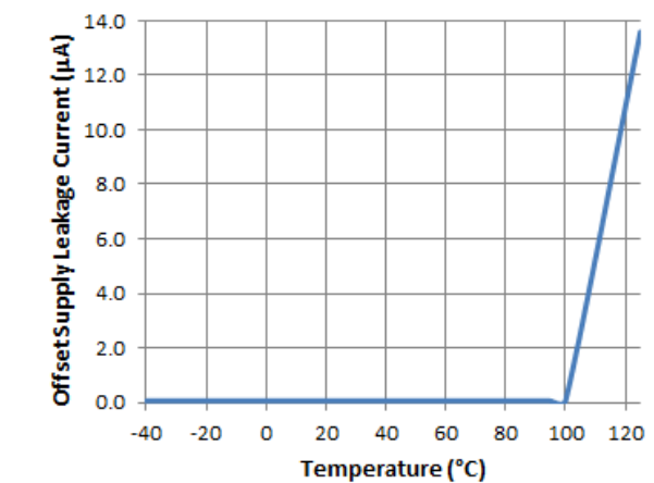
Figure 27. Offset Supply Leakage Current vs. Temperature
