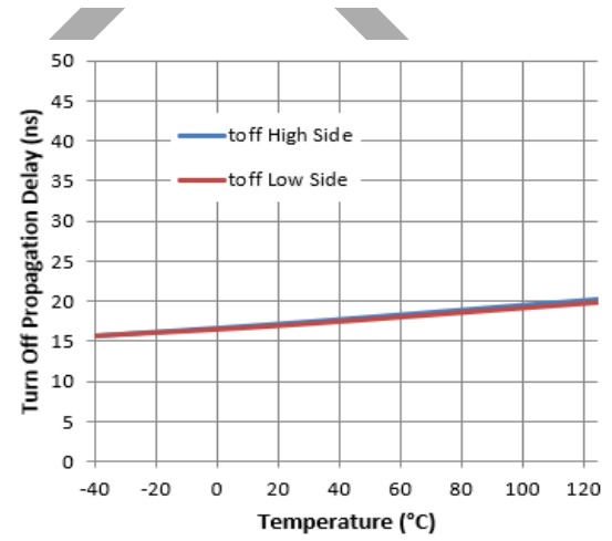
Figure 6. Turn-off Propagation Delay vs. Temperature
