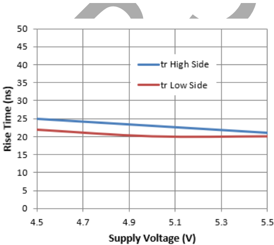
Figure 7. Rise Time vs. Supply Voltage
