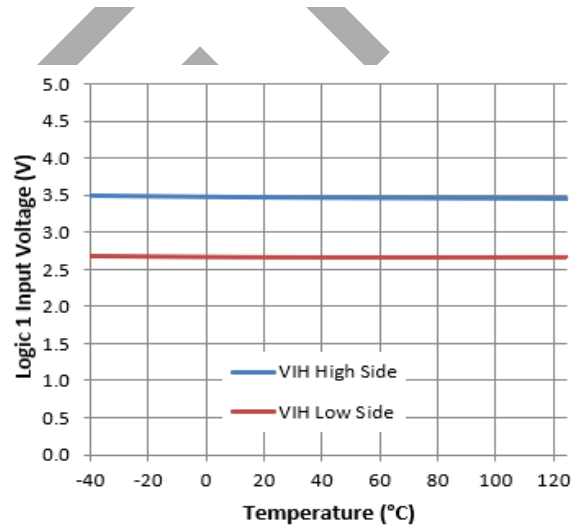
Figure 18. Logic 1 Input Voltage vs. Temperature
