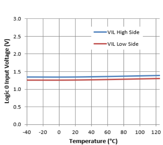
Figure 20. Logic 0 Input Voltage vs. Temperature
