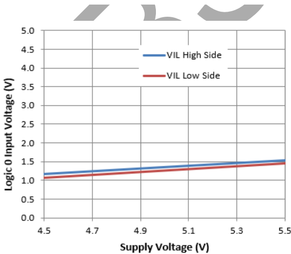
Figure 19. Logic 0 Input Voltage vs. Supply Voltage
