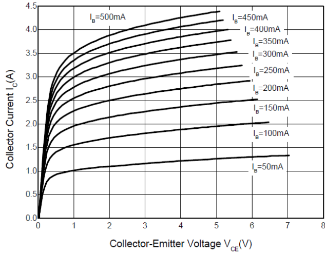
Static Characteristics
