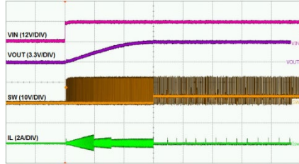
Time-5ms/div
