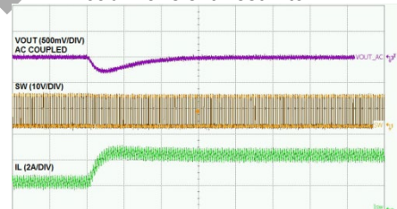
Time-50μs/div
