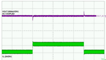
Time-2ms/div
