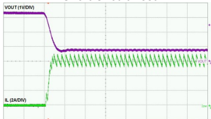
Time-50μs/div
