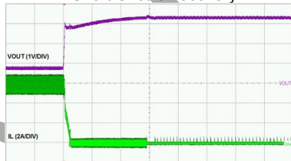
Time-2ms/div
