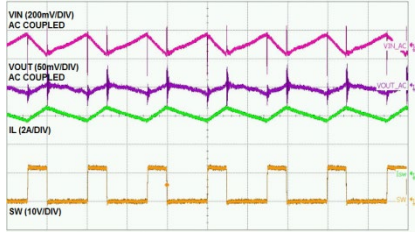
Time-2μs/div
