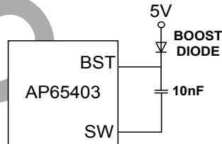
Figure 5—External Bootstrap Compensation Components
