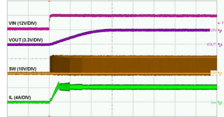
Time-5ms/div
