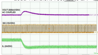
Time-50μs/div
