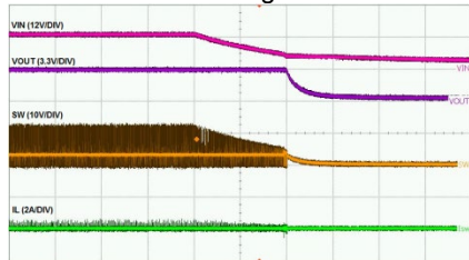
Time-100ms/div
