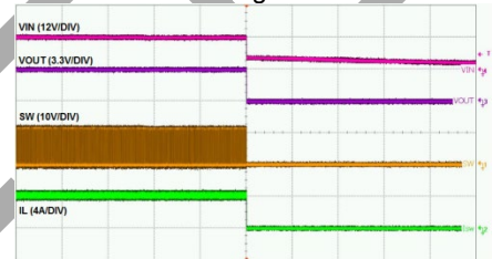
Time-100ms/div
