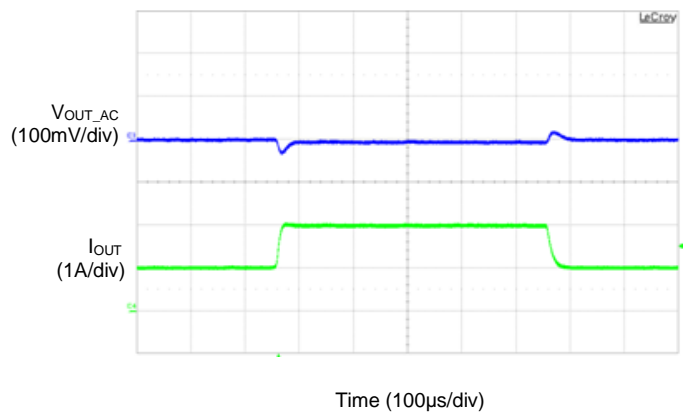
Load Transient (I OUT =1A to 2A)
