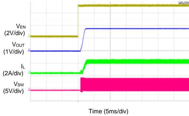
Enable Turn on Characteristic (I OUT =2A)
