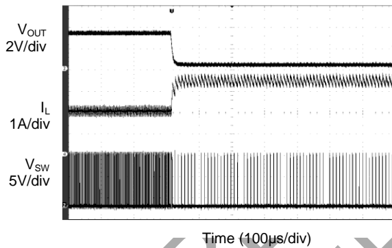
Short Circuit Protection ( I_{OUT}=2\text{A} )
