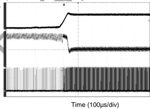
Short Circuit Recovery ( I_{OUT}=2\text{A} )
