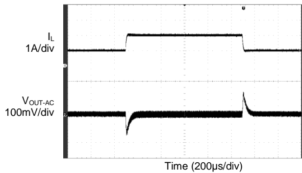
Load Transient ( I_{OUT}=1 to 2\text{A} )
