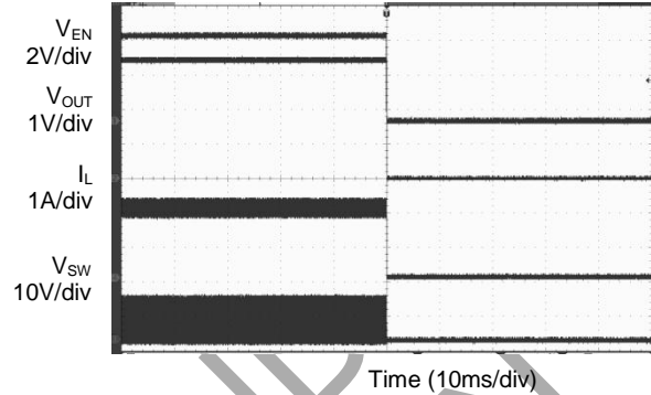
Enable Turn off Characteristic ( I_{OUT}=2\text{A} , CC Mode)
