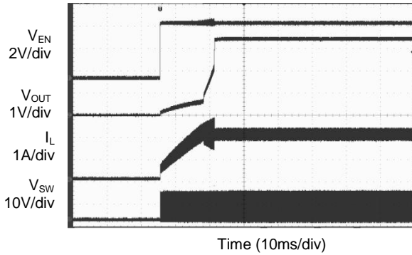
Enable Turn on Characteristic ( I_{OUT}=2\text{A} , CC Mode)
