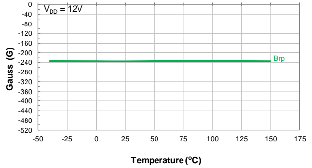
Switch Release Points Brp vs Temperature
