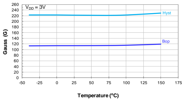
Switch Release Point Bop vs Temperature
