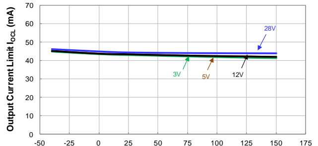
Output Current Limit vs Temperature
