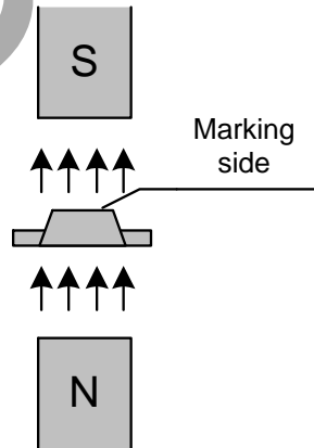
( SOT89-5L )
