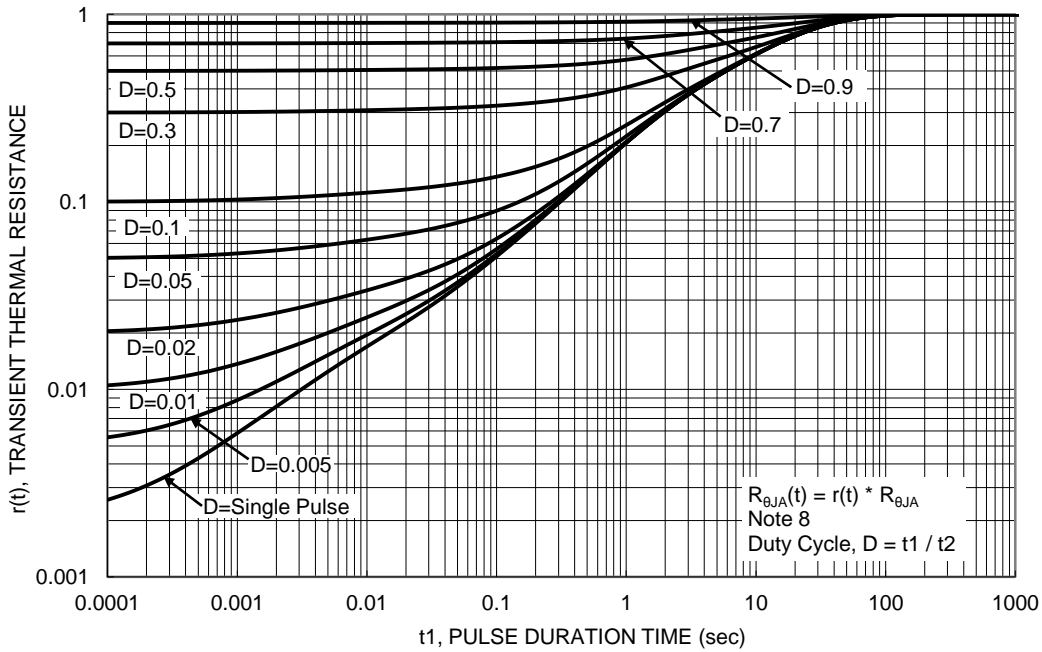
Figure 8. Transient Thermal Resistance MRP (Note 8)
