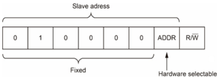
Figure 6. PI4IOE5V6416A address
