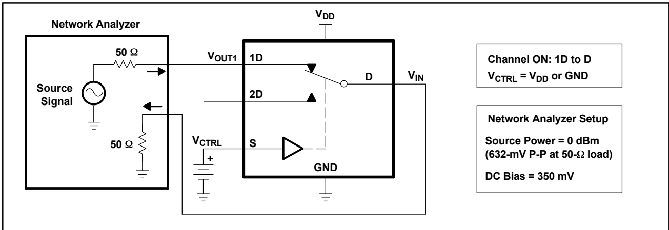
Figure 5. Bandwidth (BW)
