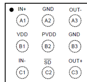
9 Ball WCSP (A) (EOL) Top View
