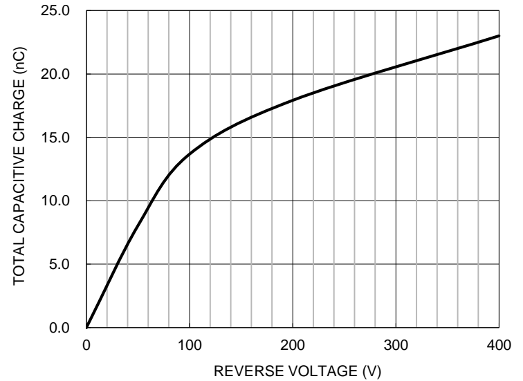
Figure 6. Typical Capacitive Charges
