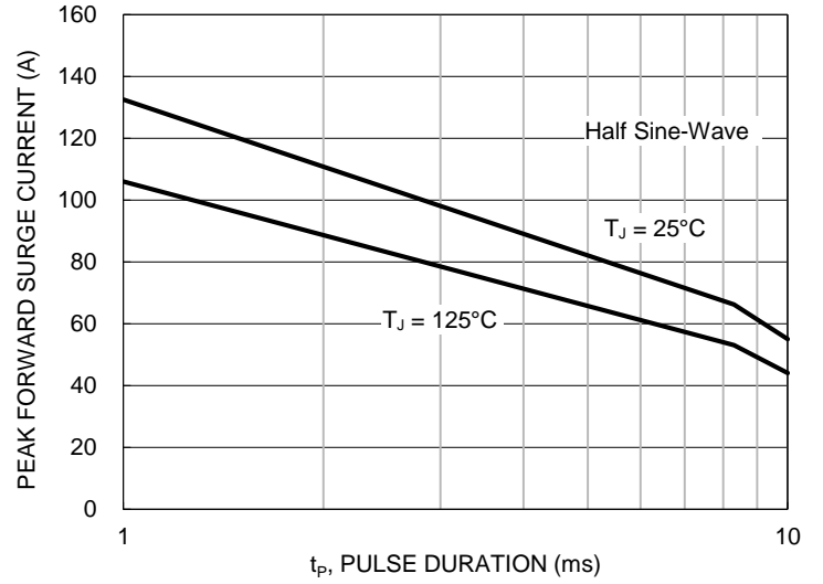
Figure 2. Non-Repetitive Peak Surge Forward Current
