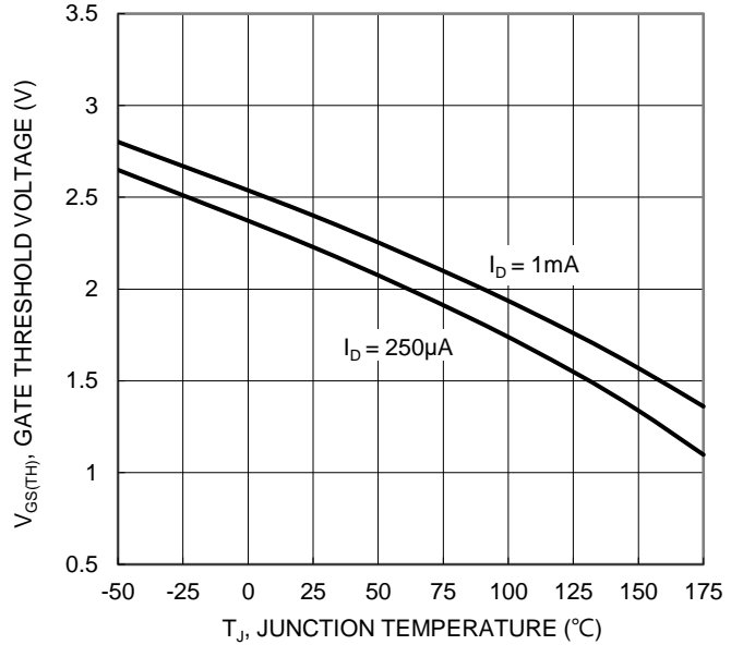
Figure 8. Gate Threshold Variation vs. Junction Temperature
