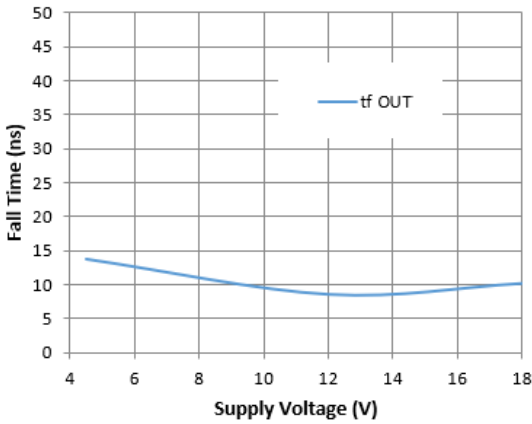
Figure 8. Fall Time vs. Supply Voltage
