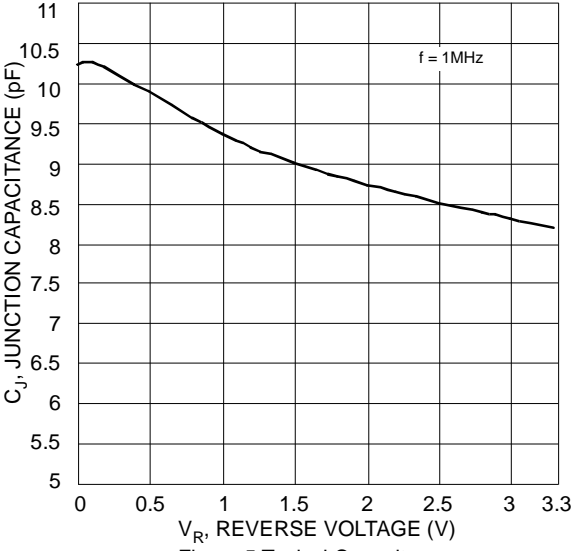
Figure 5 Typical Capacitance
