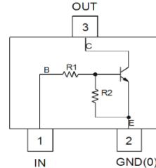
Device Schematic
