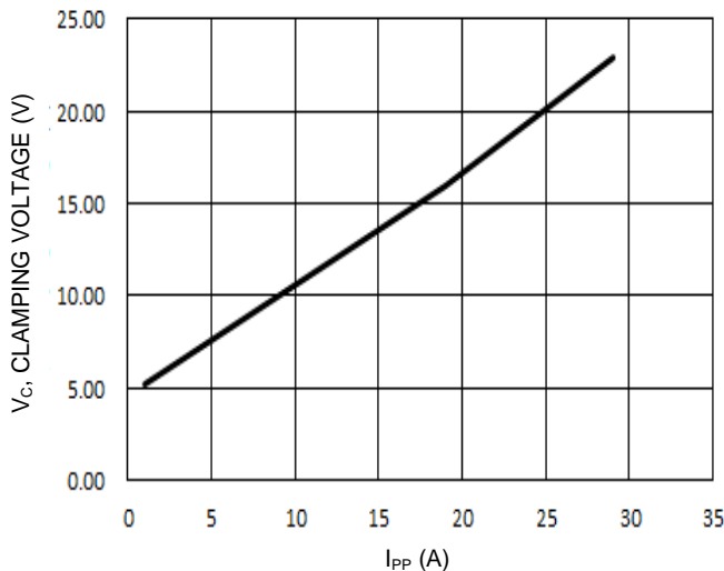
Figure 7. Clamping Voltage Characteristics ( t_p = 8/20\mu s )
