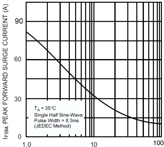
NUMBER OF CYCLES AT 60 Hz Figure 3. Maximum Peak Forward Surge Current (Per Leg)
