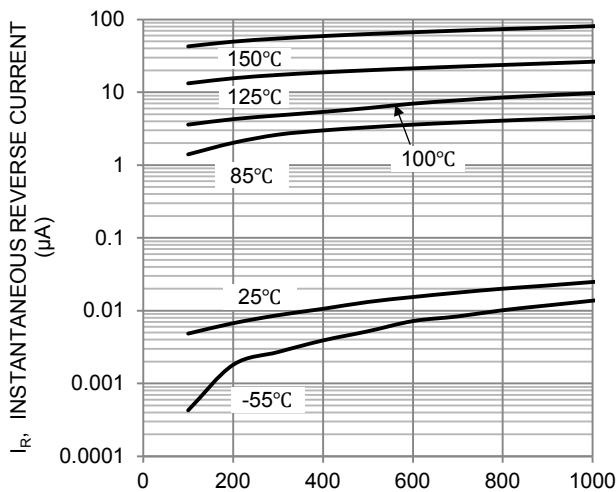
V_R , INSTANTANEOUS REVERSE VOLTAGE (V) Figure 5. Typical Reverse Characteristics (Per Leg)
