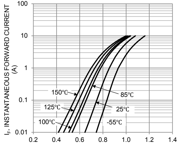
V_F , INSTANTANEOUS FORWARD VOLTAGE (V) Figure 2. Typical Forward Characteristics (Per Leg)
