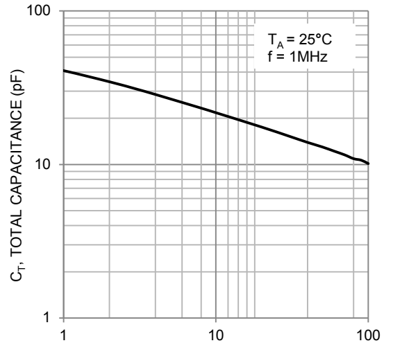
V_R , REVERSE VOLTAGE (V) Figure 4. Typical Total Capacitance (Per Leg)
