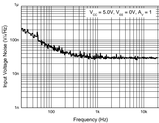
Figure 1. Input Voltage Noise in Conventional Amplifier
