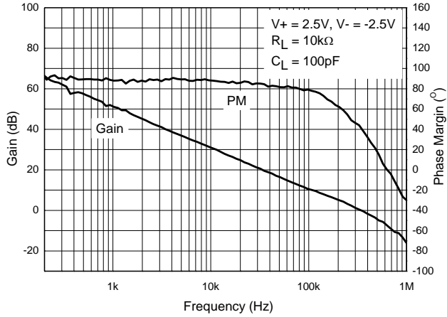
Frequency Response (Gain and Phase Margin)
