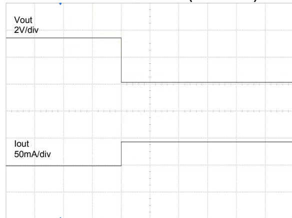
Time (1ms/div)
