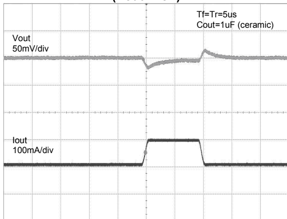
Output Load Transient Response (Vout=2.8V)
