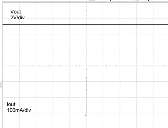
Time (50us/div)
