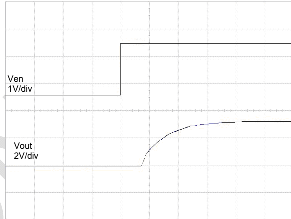
Time (20us/div)
