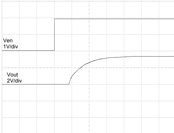
Time (20us/div)
