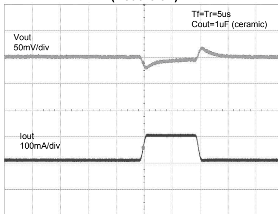
Output Load Transient Response (Vout=3.0V)
