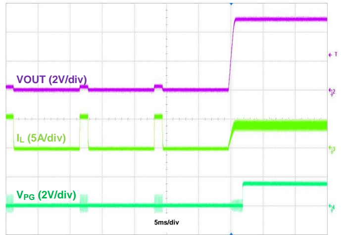
Figure 12. Output Short Recovery with PG, IOU = 4A
