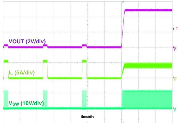
Figure 10. Output Short Recovery, IOU = 4A
