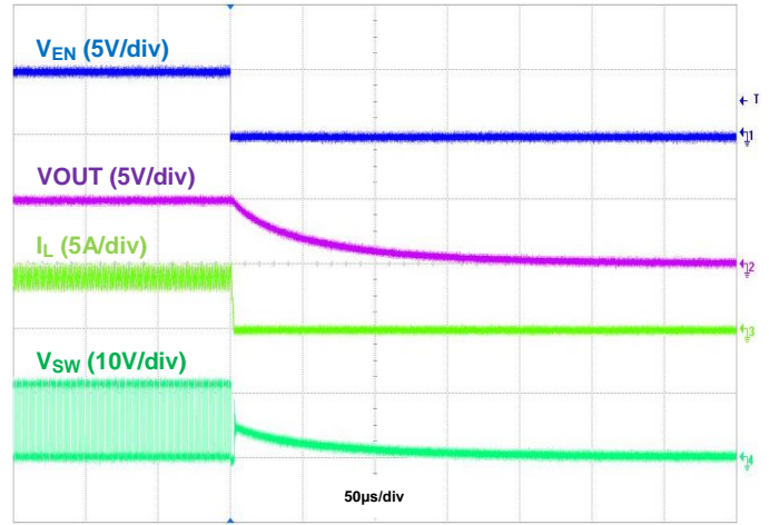
Figure 8. Shutdown Using EN, IOU = 4A
