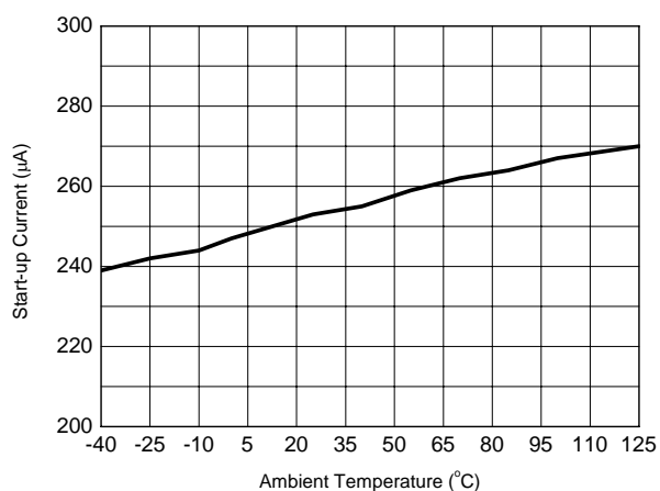
Figure 5. Start-up Current vs. Ambient Temperature
