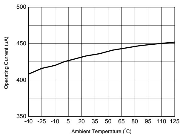
Figure 4. Operating Current vs. Ambient Temperature
