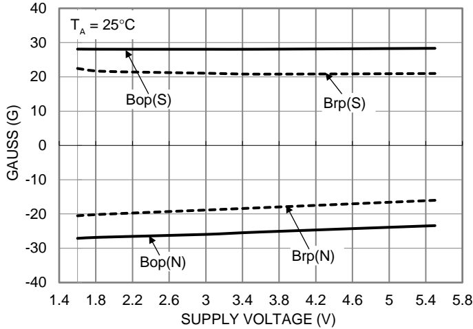
Figure 7. Switch Points vs Supply Voltage
