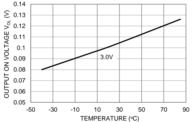
Figure 4. Output On Voltage vs. Temperature
