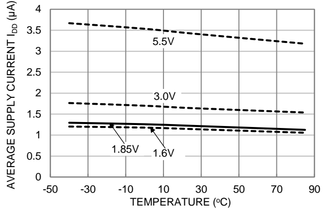
Figure 2. I_{DD(AVG)} vs. Temperature
