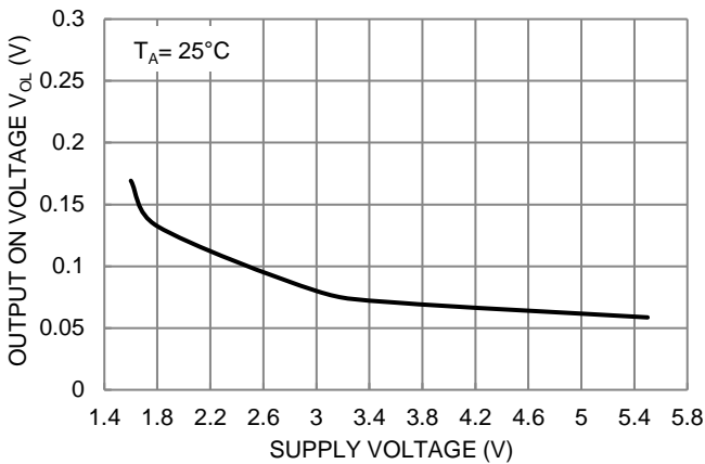
Figure 3. Output On Voltage vs. Supply Voltage
