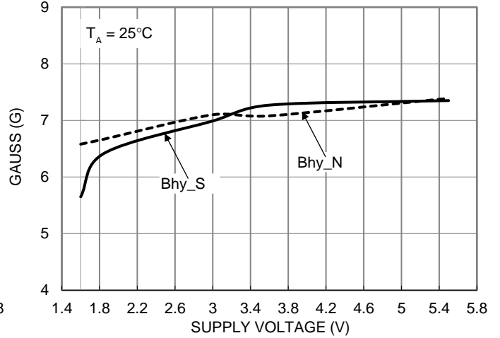
Figure 8. Hysteresis B HY vs Supply Voltage
