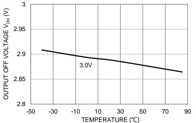
Figure 6. Output Off Voltage vs. Temperature
