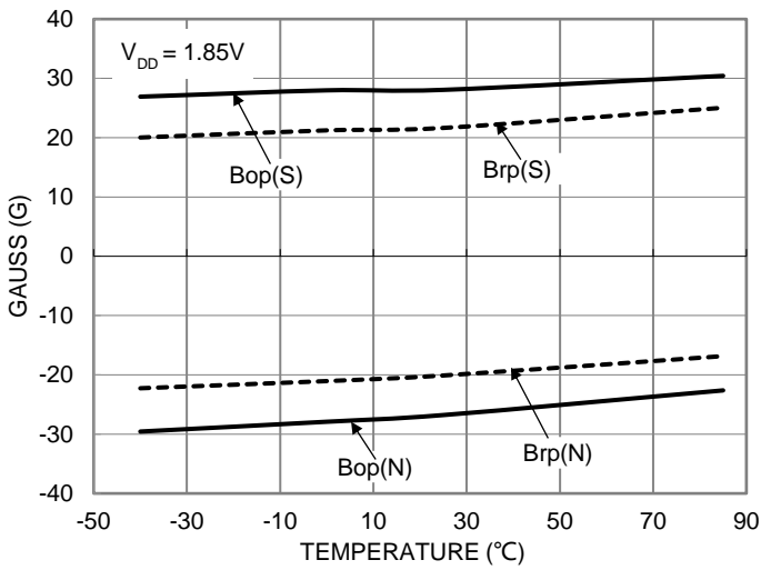
Figure 9. Switch Points vs Temperature
