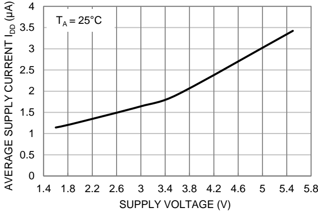
Figure 1. I_{DD(AVG)} vs. Supply Voltage
