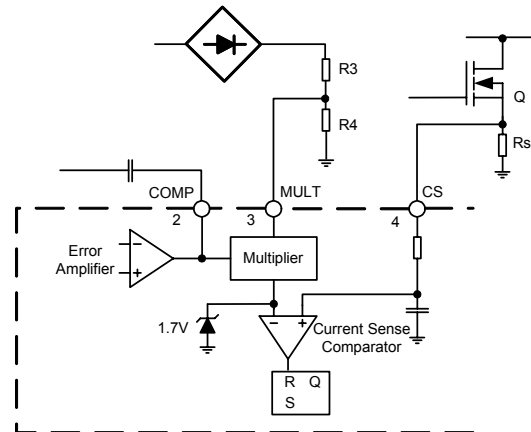
Figure 6. Multiplier Block
