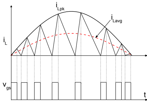
Figure 9. Boost Inductor Current in DCM Boundary Conduction Mode
